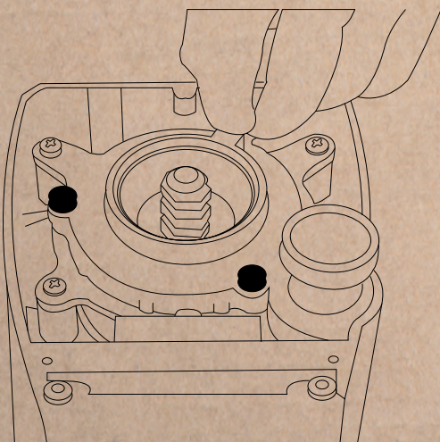
⑦ Unscrew the upper burr holder
