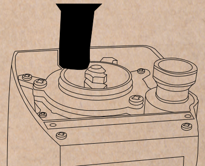
⑥ First cleaning of the grinding chamber
