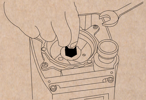
14 Unscrew and take out the lower burr
